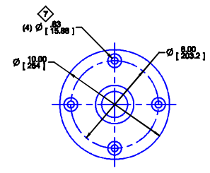
SUPPORT PIPE BASE SCALE 1:4
