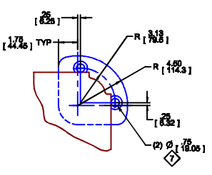
SEAMER BASE LEG FOOT 4 PLACES SCALE 1:4
