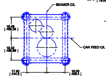
SEAMER BASE LEG CENTERS
