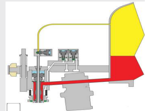
CB244 Filling Valve
