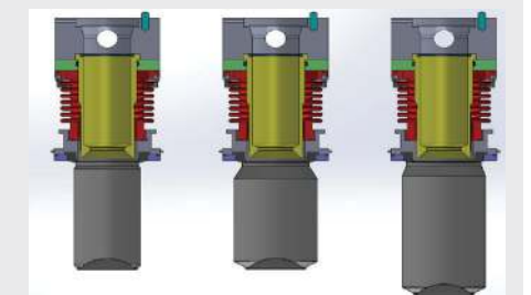
No adjustments to filling valve required for different can sizes
